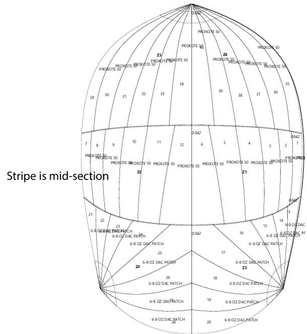
Tri-Radial Layout
